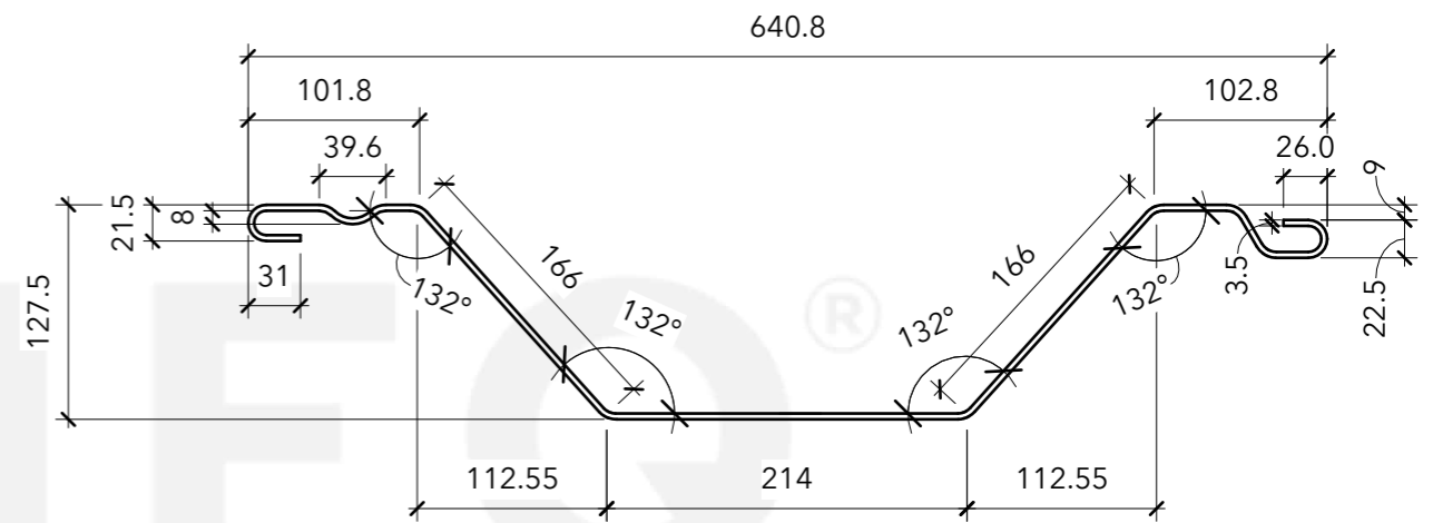
SCALE 1:5
